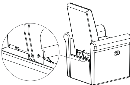
2. Pull up the backrest, connect the gas lift and backrest by pin and lock it by split cotter
