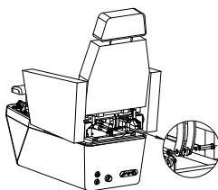
2. Install motor shaft and fix the bolt.
